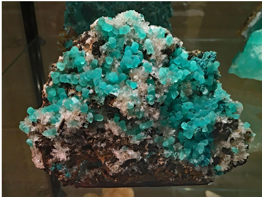
Smithsonite, San Antonio El Grande Mine, Chihuahua, Mexico
